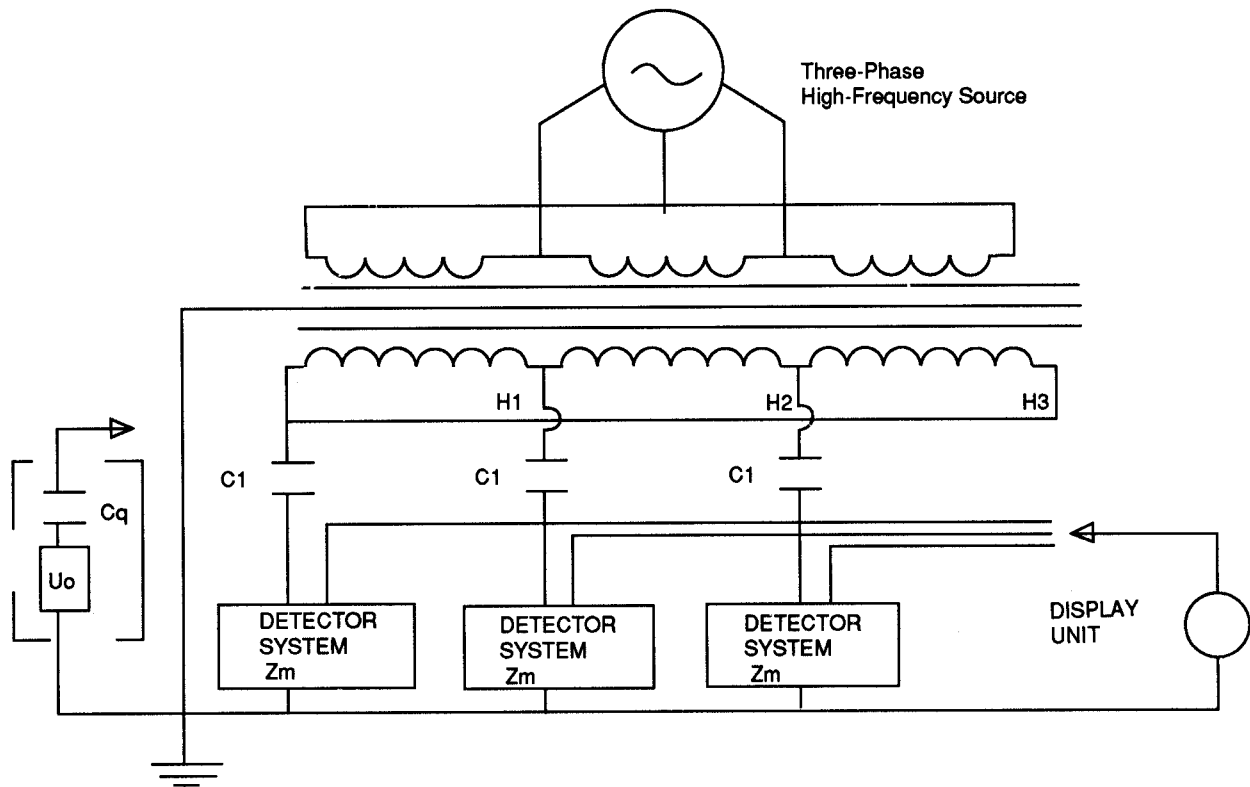
Figure 5— Induced Voltage Balanced Winding
