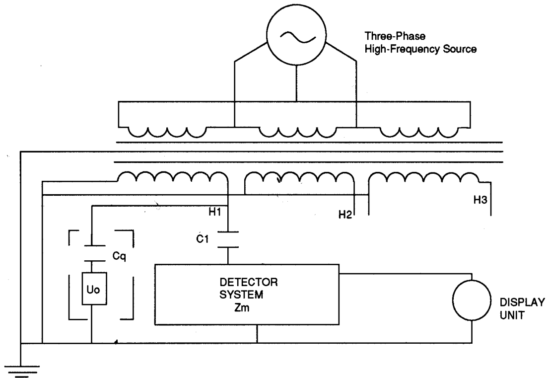
Figure 8— Induced Voltage Wye Connect With Neutral Grounded and the Detector on Line Terminal
