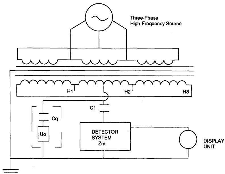
Figure 7— Induced Voltage Center Grounded Through the Detector System
