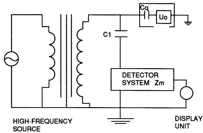
Figure 2— Induced Voltage One End of Transformer Grounded or Ground Wye Transformer
