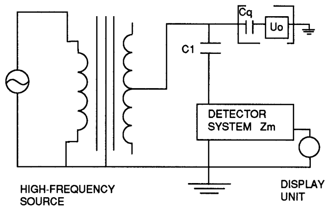
Figure 4— Induced Voltage Center Winding
