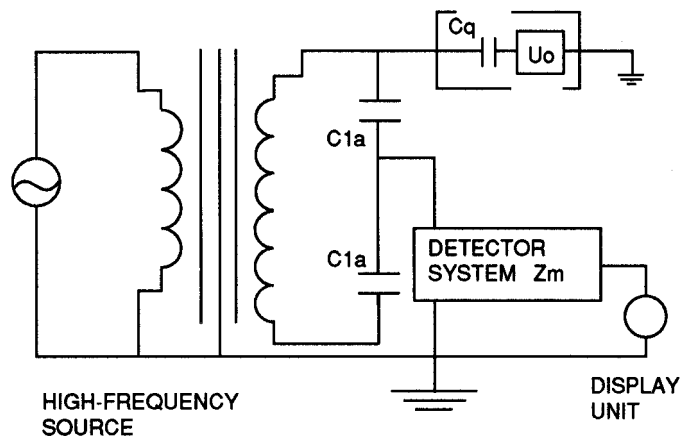
Figure 3— Induced Voltage Balanced Winding
