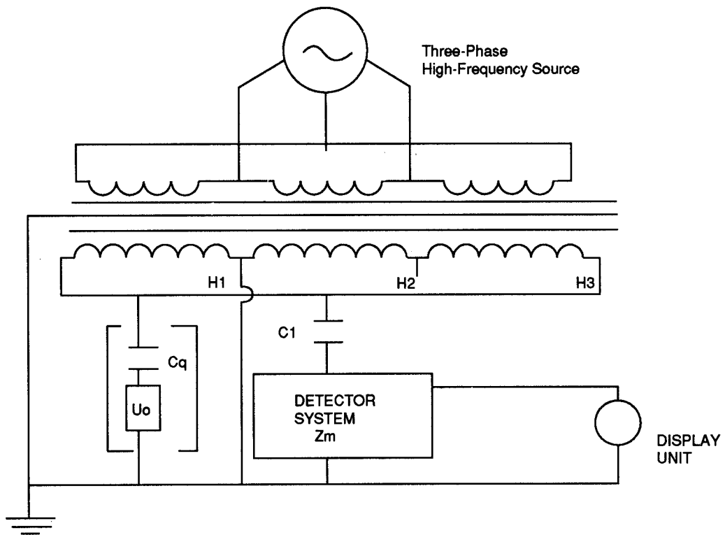
Figure 6— Induced Voltage One Corner Grounded
