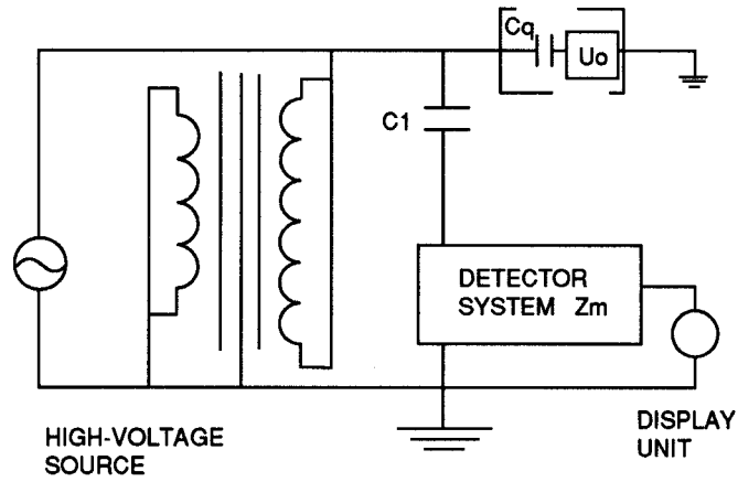
Figure 1— Applied Voltage
