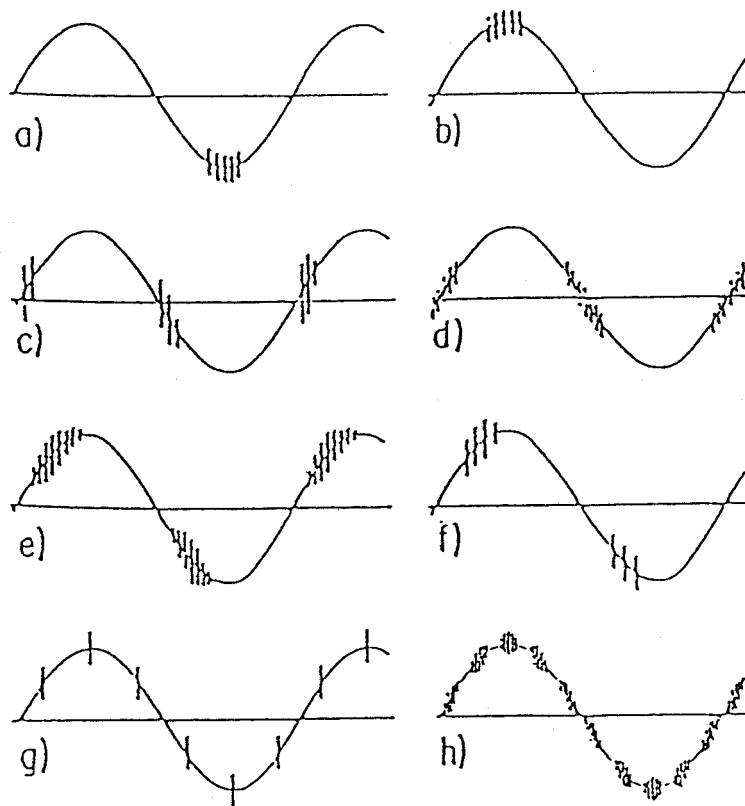
Figure A1 —Oscilloscope Response of Partial Discharge
